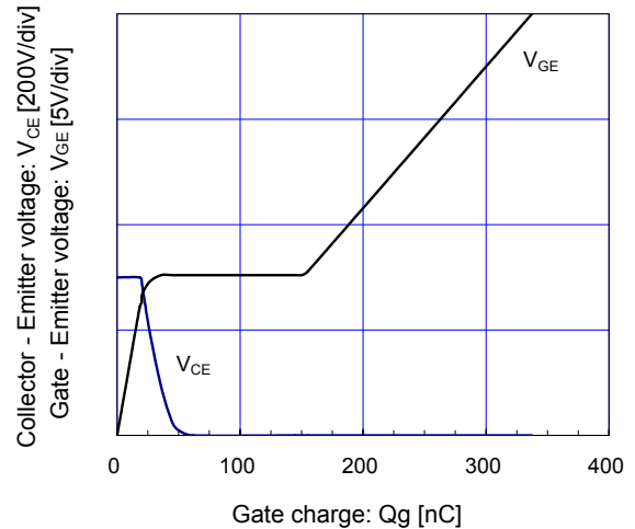
[ Brake ] Dynamic gate charge (typ.) V_{CC} = 300\text{V} , I_c = 50\text{A} , T_j = 25^\circ\text{C}
